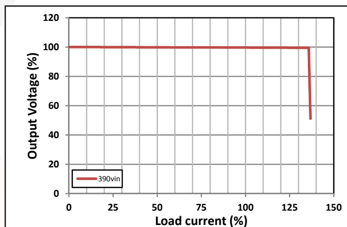
Figure 6: Output voltage vs. load current showing typical current limit curves. See Current limit section in application notes.
