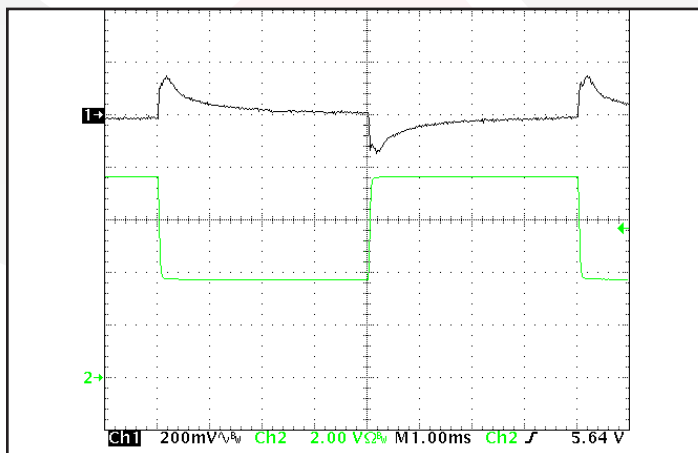
Figure 11: Output voltage response to step-change in load current 50%-100%-50% of Iout (max); dI/dt = 0.07 A/μs. No external load capacitance. Ch 1: Vout (200 mV/div). Ch 2: Iout (2 A/div). (1 ms/div).
