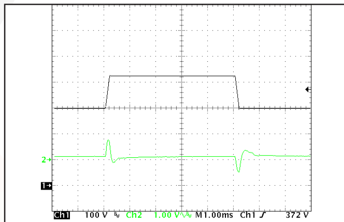
Figure 12: Output voltage response to step-change in input voltage (300 V - 425 V - 300 V); dV/dt = 800 V/ms. Ch 1: Vin (100 V/div). Ch 2: Vout (1 V/div). (1 ms/div).
