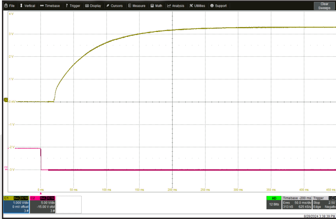
Figure 7: Turn-on transient at full load and zero output capacitance initiated by On/Off. Input voltage pre-applied. Ch 1: Vout (1 V/div). Ch 2: On/Off (5 V/div). Timescale: 50.0 ms/div.
