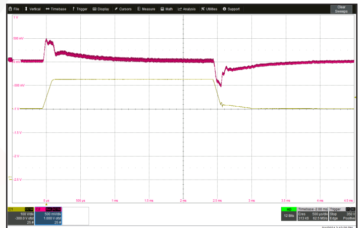
Figure 12: Output voltage response to step-change in input voltage (300 V - 425 V - 300 V) in 125 μs. Ch 1: Vin (100 V/div). Ch 2: Vout (500 mV/div). Timescale: 500 μs/div.
