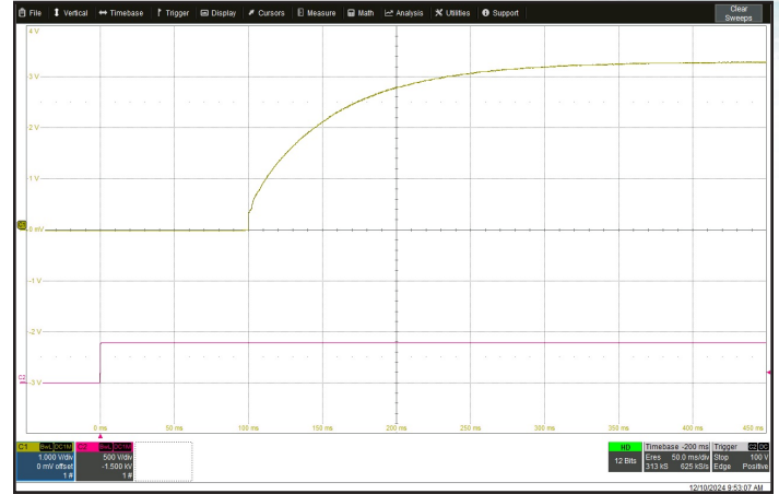
Figure 8: Turn-on transient at full load and zero output capacitance initiated by Vin. On/Off Pin previously low. Ch 1: Vout (1 V/div). Ch 2: Vin (500 V/div). Timescale: 50.0 ms/div.
