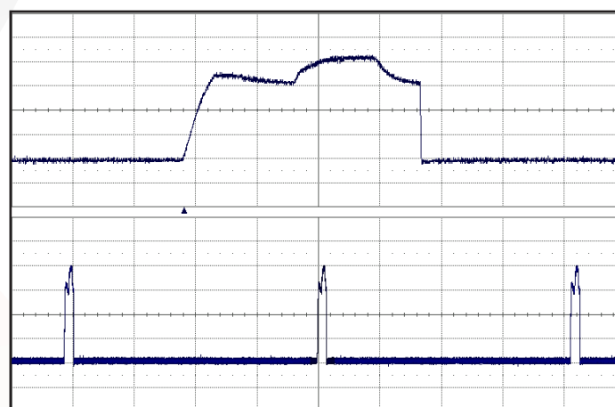
Figure 18: Load current (20A/div) as a function of time (2ms/div and 50ms/div) when the converter attempts to turn on into a 10 mΩ short circuit.
