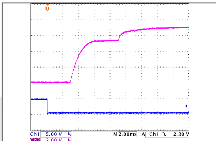
Figure 7: Typical startup waveform. Input voltage pre-applied, ON/OFF Pin. Ch 1: ON/OFF Pin (5V/div). Ch 3: Vout (2V/div).
