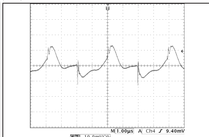
Figure 10: Output voltage ripple, Vout, at nominal input voltage and rated load current (10 mV/div). Load capacitance: 1μF ceramic capacitor and 10μF tantalum capacitor. Bandwidth: 10 MHz. See Figure 17.
