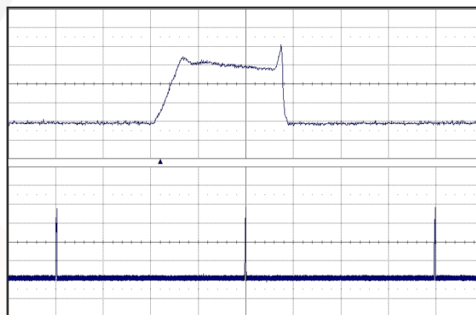
Figure 18: Load current (10A/div) as a function of time (0.5ms/div and 50ms/div) when the converter attempts to turn on into a 10 mΩ short circuit.
