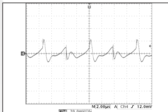
Figure 10: Output voltage ripple, Vout, at nominal input voltage and rated load current (20 mV/div). Load capacitance: 1μF ceramic capacitor and 10μF tantalum capacitor. Bandwidth: 10 MHz. See Figure 17.
