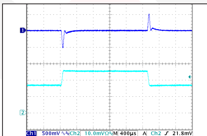
Figure 11: Output voltage response to step-change in load current (50%-75%-50% of I_{out(max)} ; dI/dt = 0.1 A/\mu s ). Load cap: 1 μF ceramic and 15 μF tantalum capacitors. Ch 1: Vout (500mV/div), Ch 2: Iout (10A/div).
