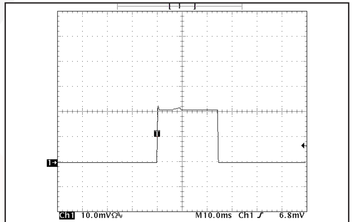
Figure 18: Load current (5A/div) as a function of time (10ms/div and 100ms/div) when the converter attempts to turn on into a 1 mΩ short circuit.
