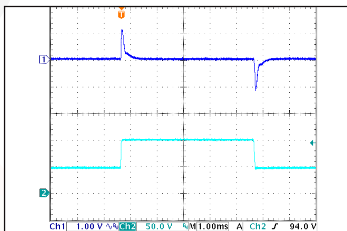
Figure 12: Output voltage response to step-change in input voltage (250V/ms). Load cap: 100 µF electrolytic output capacitance. Ch 1: Vout (1V/div), Ch 2: Vin (50V/div).
