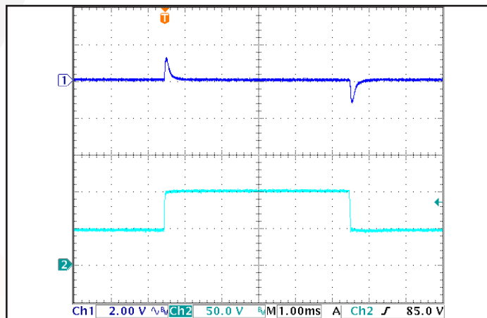
Figure 12: Output voltage response to step-change in input voltage (250V/ms). Load cap: 100 μF electrolytic output capacitance. Ch 1: Vout (2V/div), Ch 2: Vin (50V/div).
