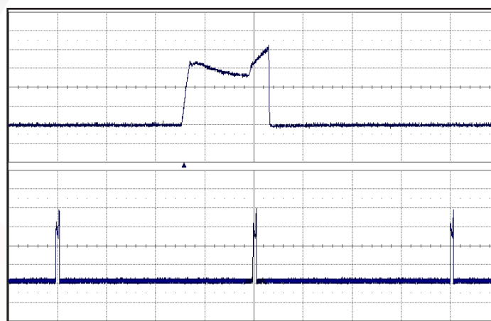
Figure 18: Load current (5A/div) as a function of time (2ms/div and 50ms/div) when the converter attempts to turn on into a 10 mΩ short circuit.
