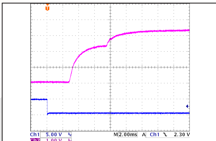
Figure 7: Typical startup waveform. Input voltage pre-applied, ON/OFF Pin. Ch 1: ON/OFF Pin (5V/div). Ch 3: Vout (1V/div), (2ms/div).
