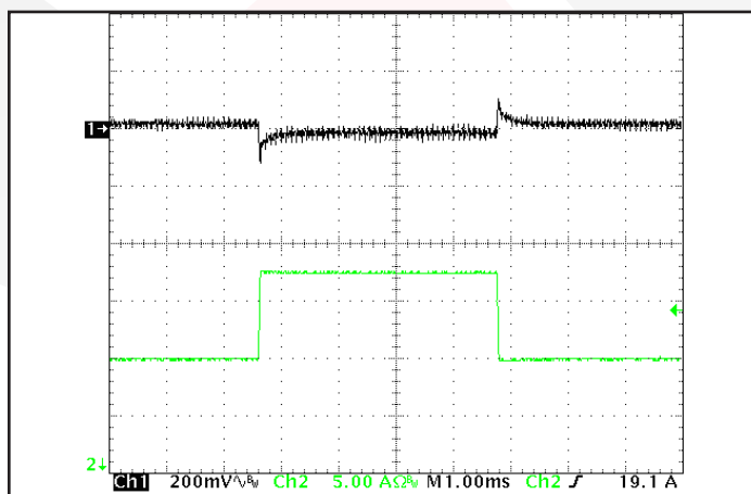
Figure 11: Output voltage response to step-change in load current (50%-75%-50% of I_{out(max)} ; dI/dt = 0.1 A/μs ). Load cap: 1 μF ceramic and 15 μF tantalum capacitors. Ch 1: Vout (200mV/div), Ch 2: Iout (5A/div), (1ms/div).
