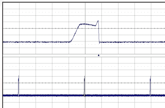
Figure 18: Load current (20A/div) as a function of time (1ms/div and 50ms/div) when the converter attempts to turn on into a 10 mΩ short circuit.
