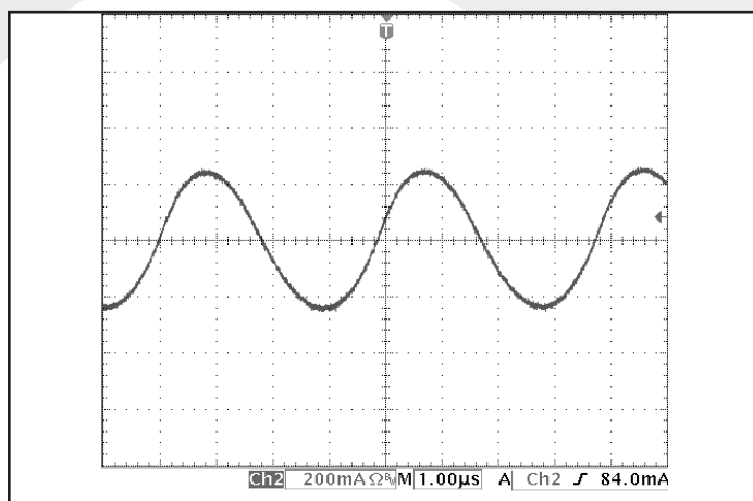
Figure 9: Input terminal current ripple, i_C , at full rated output current and nominal input voltage with SynQor MCOTS filter module (200 mA/div). Bandwidth: 20MHz. See Figure 17, (1μs/div).
