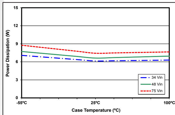
Figure 4: Power dissipation at nominal output voltage and 66% rated power vs. case temperature for minimum, nominal, and maximum input voltage.
