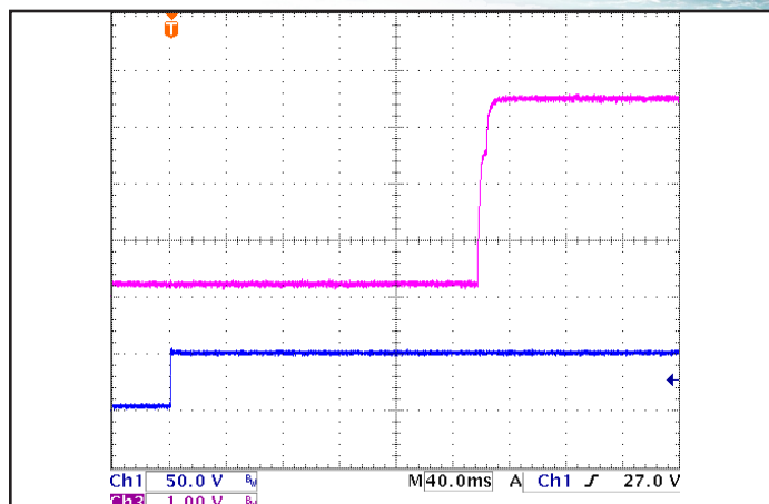
Figure 8: Turn-on transient at full resistive load and zero output capacitance initiated by Vin. ON/OFF Pin previously low. Ch 1: Vin (50V/div). Ch 3: Vout (1V/div), (40ms/div).
