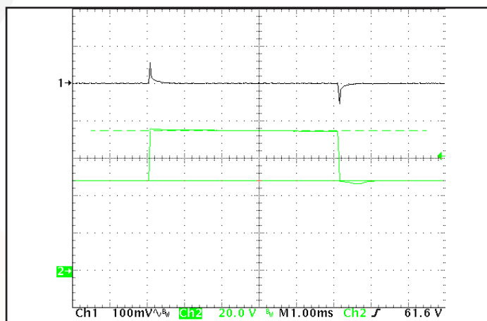
Figure 12: Output voltage response to step-change in input voltage (250V/ms). Load cap: 100 μF electrolytic output capacitance. Ch 1: Vout (100mV/div), Ch 2: Vin (20V/div), (1ms/div).
