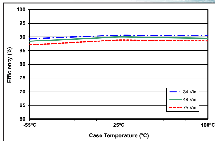
Figure 2: Efficiency at nominal output voltage and 66% rated power vs. case temperature for minimum, nominal, and maximum input voltage.
