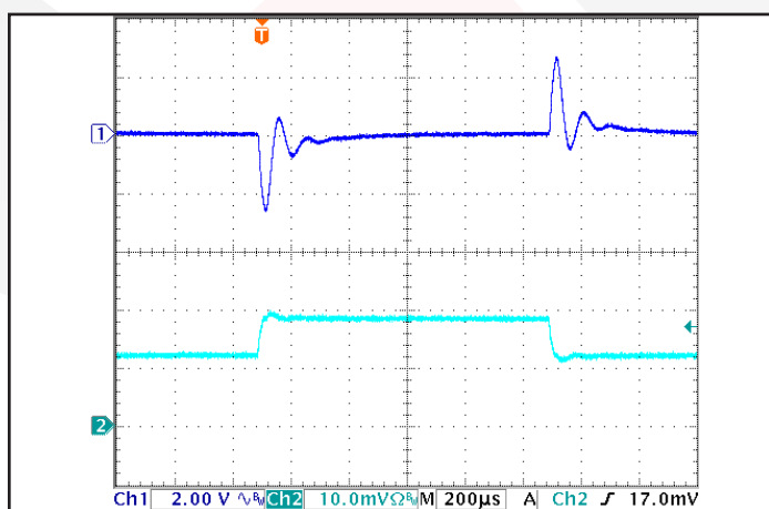
Figure 11: Output voltage response to step-change in load current (50%-75%-50% of I_{out(max)} ; dI/dt = 0.1 A/\mu s ). Load cap: 1 μF ceramic and 15 μF tantalum capacitors. Ch 1: Vout (2V/div), Ch 2: Iout (2A/div).
