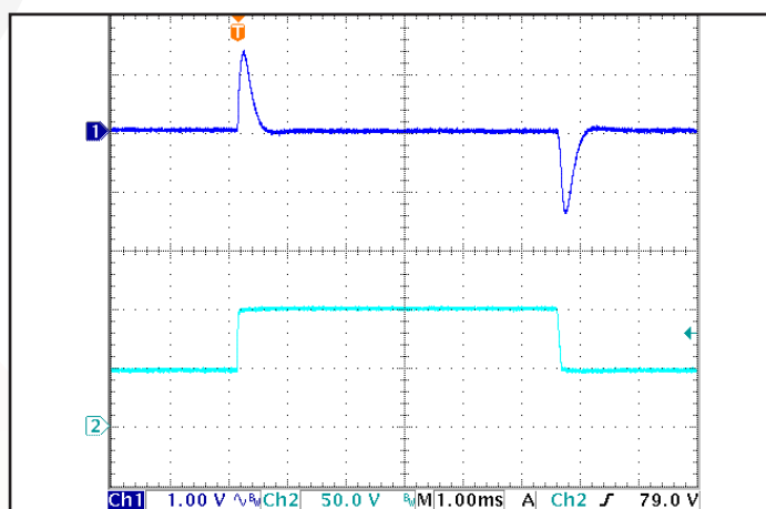
Figure 12: Output voltage response to step-change in input voltage (250V/ms). Load cap: 100 μF electrolytic output capacitance. Ch 1: Vout (1V/div), Ch 2: Vin (50V/div).
