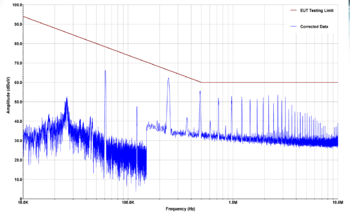
Figure 2: MIL-STD-461F Method CE102 High Frequency Conducted Emissions. Limit line (in red) is the 'Basic Curve'.
