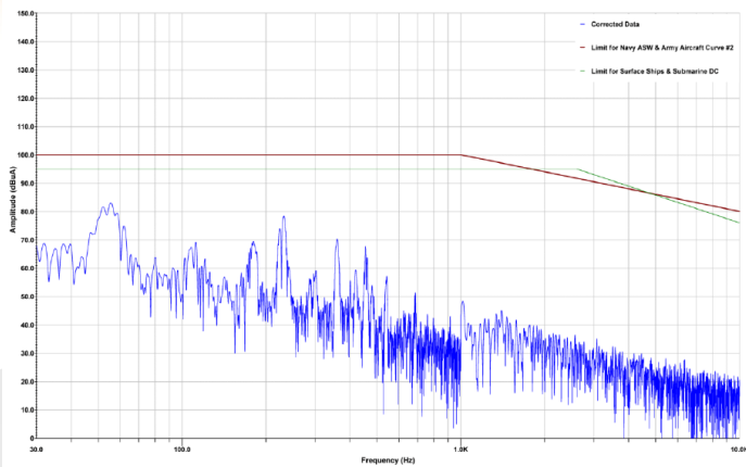
Figure 1: MIL-STD-461F Method CE101 Low Frequency Conducted Emissions.
