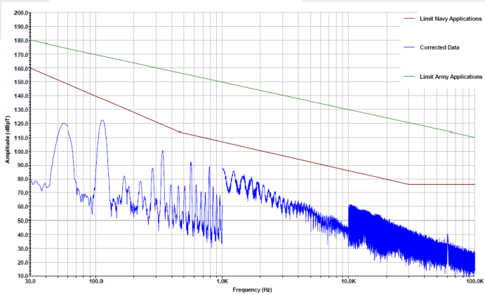
Figure 3: MIL-STD-461F Method RE101 Low Frequency Radiated Emissions.
