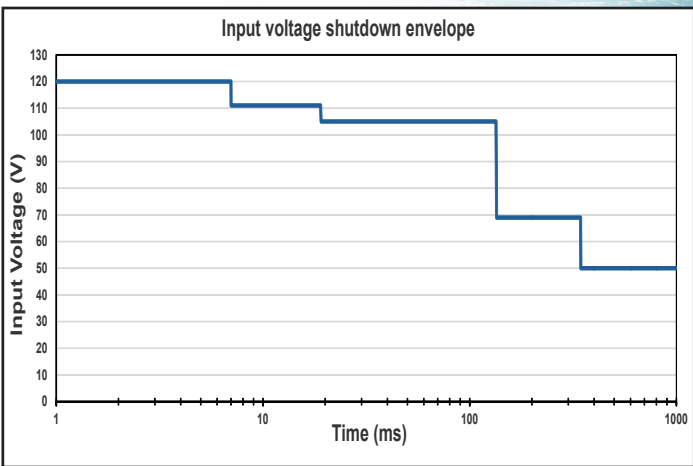
Figure E: Input Over Voltage shutdown envelope as function of time.
