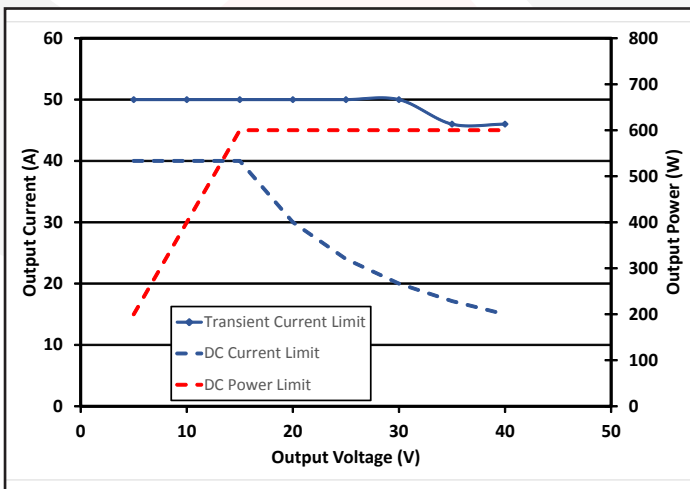
Figure C: Output Power / Current Limit as a function of Output Voltage.
