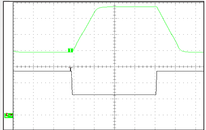
Figure 10: Output Voltage vs. Vset pin voltage dynamics; 48Vin, 5A out (10ms/div). Bottom trace: Vset pin voltage (500mV/div). Top trace: Output Voltage (10V/div).
