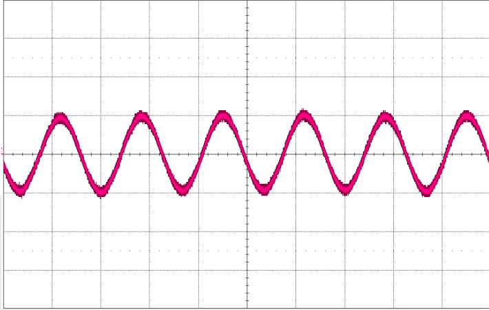
Figure 7: Output voltage ripple with 400µF Hold-up capacitor at full rated power (115VAC, 60Hz) Vout (5V/div), Timebase: (5ms/div)
