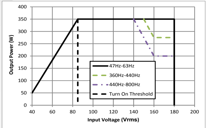
Figure 10: Continuous output power vs. input voltage, output turn-on threshold is 85Vrms
