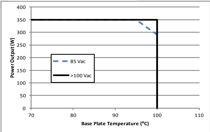
Figure 9: Output power vs. baseplate temperature derating curve
