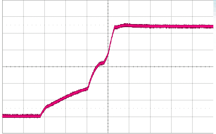
Figure 8: Output voltage startup waveform with 400µF hold-up capacitor, no load (115VAC, 60Hz), (50V/div), Timebase: (500ms/div)
