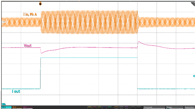
Figure 11: Responses to 25%-75%-25% load transient steps: Cext=10mF. 100 ms/div.
