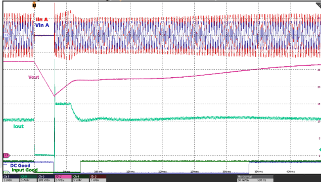
Figure 14: 30 ms power interruption and recovery. 400Hz AC in, 10A out, Cext=27mF. 50ms/div.
