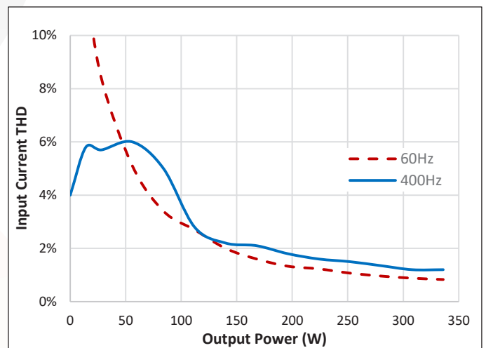
Figure 3: Input current THD over full load range at 115 Vrms (L-N). Includes MACF-115-3PH-UNV-QG external input filter module.
