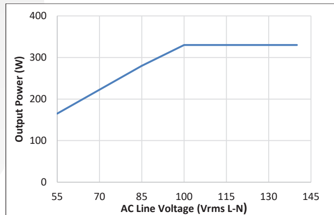
Figure 13: Steady-state rated and limit output power vs. AC line voltage.
