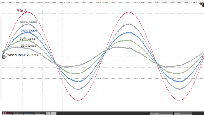
Figure 5: Typical 400 Hz input current waveforms (Phase A shown) at 25%, 50%, 75%, and 100% load. Includes currents in an MACF-115-3PH-UNV-QG external input filter module. 500μs/div.
