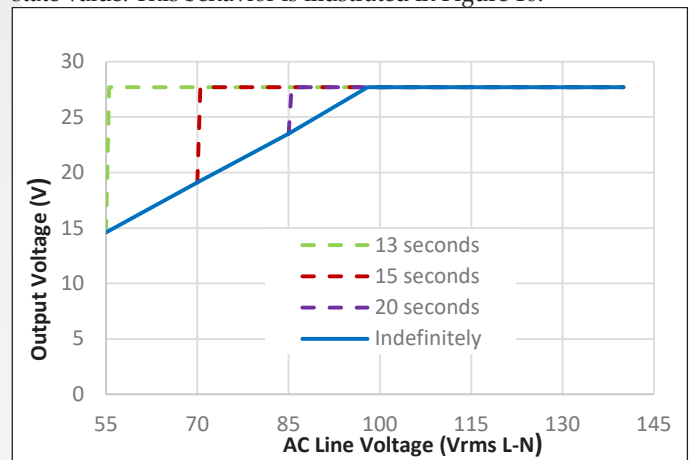
Figure 10: Full Load Output Voltage during Line Brownouts
