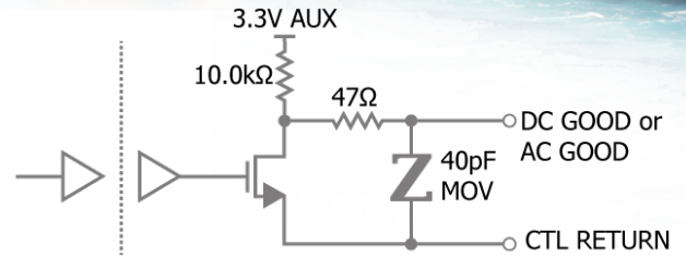
Figure 20: Internal circuitry for AC GOOD and DC GOOD pins.
