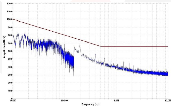
Figure 15: CE102 data at 400 Hz, 750 W output power (Phase A)
