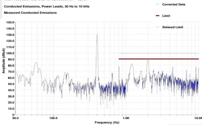
Figure 14: CE101 data at 400 Hz, 750 W output power (Phase C)
