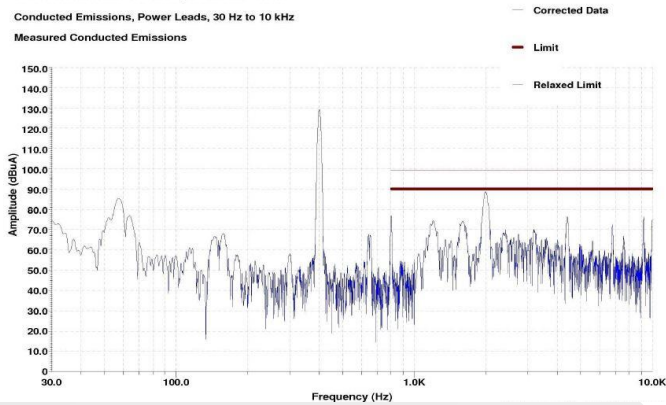
Figure 13: CE101 data at 400 Hz, 750 W output power (Phase B)
