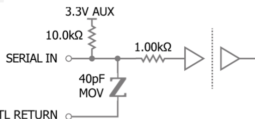
Figure 18: Internal circuitry for SERIAL IN pin.
