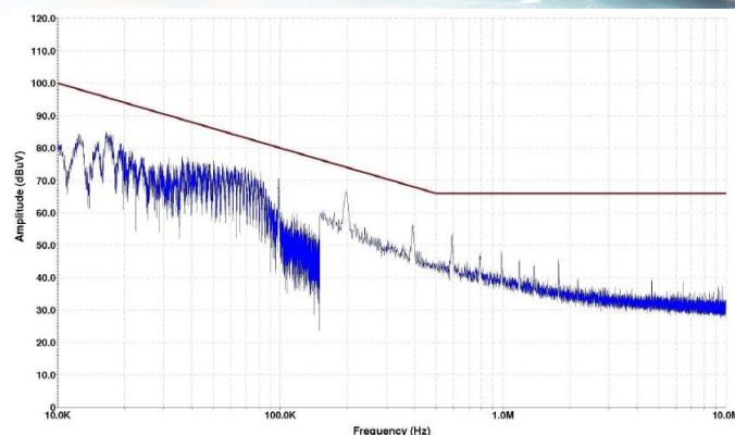
Figure 16: CE102 data at 400 Hz, 750 W output power (Phase B)
