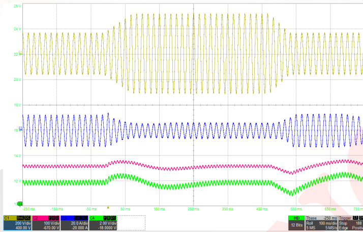
Figure 7: Input transient with 600µF hold-up capacitor at full load (115Vrms-220Vrms-115Vrms, 60Hz) Ch1: Vin (200V/div), Ch2: Vhold-up (100V/div), Ch3: Iin (20A/div), Ch4: Vout (2V/div), Timebase: (100ms/div).
