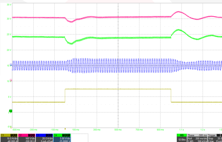
Figure 5: Load transient with 600 \mu\text{F} hold-up capacitor (50%-75%-50% of I_{\text{max}} , 115Vrms, 60Hz) Ch1: Iout (10A/div), Ch2: Hold-up voltage (100V/div), Ch3: Iin (20A/div), Ch4: Vout (5V/div), Timebase: (200ms/div).
