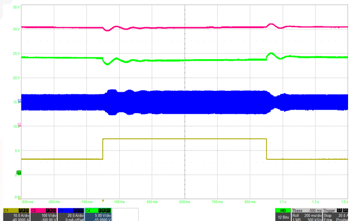
Figure 6: Load transient with 600 \mu\text{F} hold-up capacitor (50%-75%-50% of I_{\text{max}} , 115Vrms, 400Hz) Ch1: Iout (10A/div), Ch2: Hold-up voltage (100V/div), Ch3: Iin (20A/div), Ch4: Vout (5V/div), Timebase: (200ms/div).
