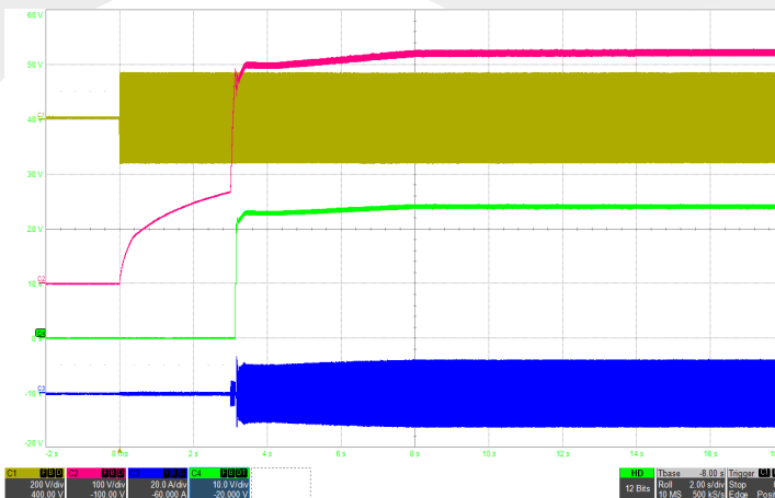
Figure 3: Typical startup waveform with 600 \mu\text{F} hold-up capacitor (115Vrms, 60Hz) Ch1: Vin (200V/div), Ch2: Hold-up capacitor voltage (100V/div), Ch3: Iin (20A/div), Ch4: Vout (10V/div), Timebase: (2s/div).
