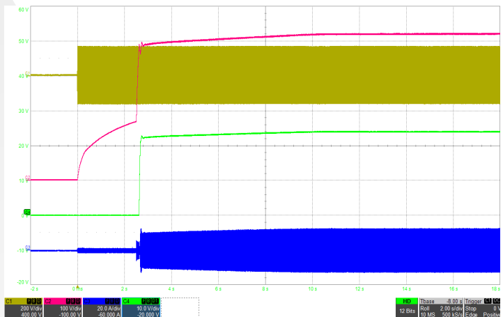
Figure 4: Typical startup waveform with 600 \mu\text{F} hold-up capacitor (115Vrms, 400Hz) Ch1: Vin (200V/div), Ch2: Hold-up capacitor voltage (100V/div), Ch3: Iin (20A/div), Ch4: Vout (10V/div), Timebase: (2s/div).
