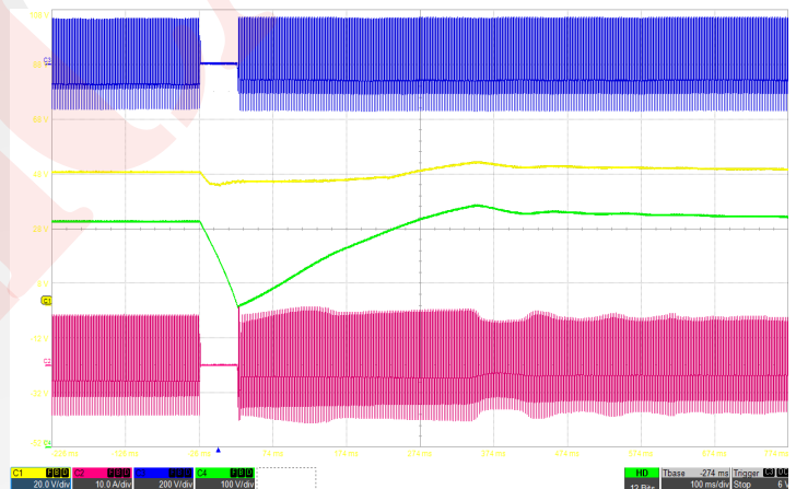
Figure 10: Line drop out with 600µF hold-up capacitor at full load (115Vrms, 400Hz) Ch1: Vout (20V/div), Ch2: Iin (10A/div), Ch3: Vin (200V/div), Ch4: Vhold-up (100V/div), Timebase: (100ms/div).
