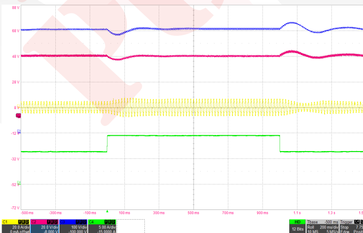
Figure 5: Load transient with 600µF hold-up capacitor (50%-75%-50% of I_{max} , 115Vrms, 60Hz) Ch1: I_{in} (20A/div), Ch2: V_{out} (20V/div), Ch3: Hold-up capacitor voltage (100V/div), Ch4: I_{out} (5A/div), Timebase: (200ms/div).
