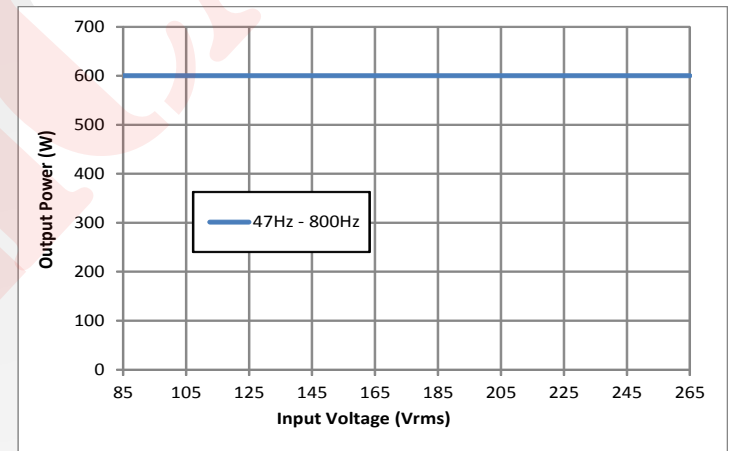
Figure 16: Maximum output power vs. input voltage at different input voltages.
