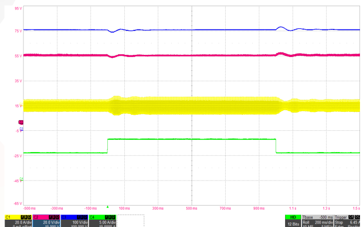
Figure 6: Load transient with 600 \mu\text{F} hold-up capacitor (50%-75%-50% of I_{\text{max}} , 115Vrms, 400Hz) Ch1: Iin (20A/div), Ch2: Vout (20V/div), Ch3: Hold-up capacitor voltage (100V/div), Ch4: Iout (5A/div), Timebase: (200ms/div).
