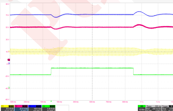
Figure 5: Load transient with 600 \mu\text{F} hold-up capacitor (50%-75%-50% of I_{\text{max}} , 115Vrms, 60Hz) Ch1: Iin (20A/div), Ch2: Vout (20V/div), Ch3: Hold-up capacitor voltage (100V/div), Ch4: Iout (5A/div), Timebase: (200ms/div).
