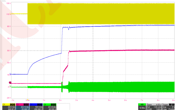
Figure 4: Typical startup waveform with 600 \mu\text{F} hold-up capacitor (115Vrms, 400Hz) Ch1: Vin (200V/div), Ch2: Vout (20V/div), Ch3: Hold-up capacitor voltage (100V/div), Ch4: Iin (20A/div), Timebase: (1s/div).
