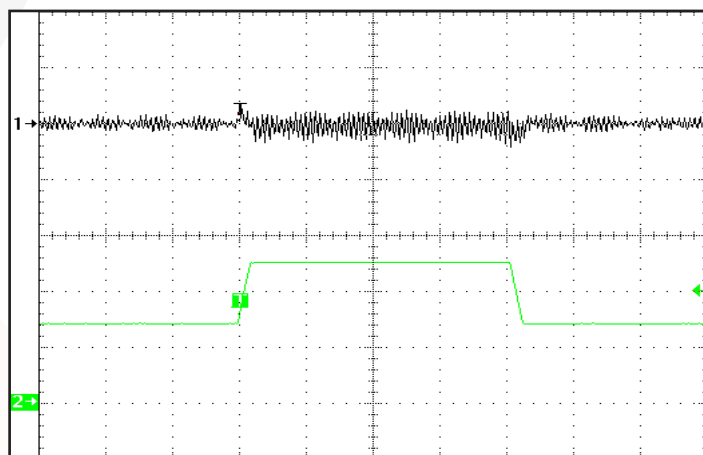
Figure 12: Output voltage response to step-change in input voltage (28V - 50V - 28V) in 150μs (50μs/Div). Ch 1: Vout (50mV/div). Ch 2: Vin (20V/div).
