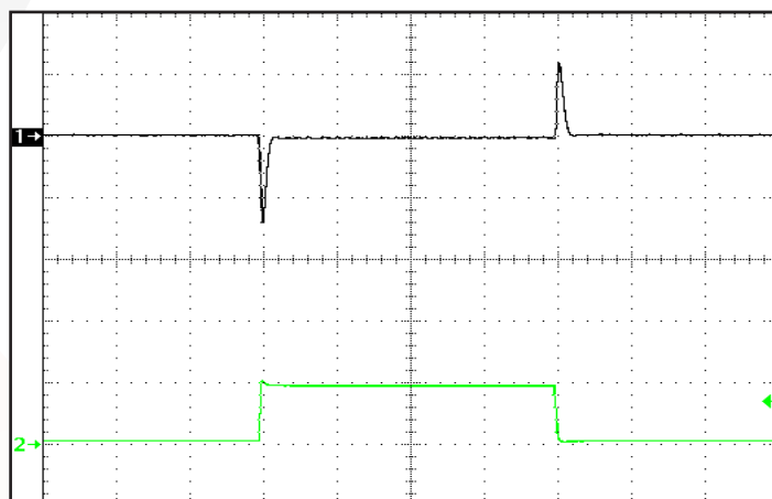
Figure 12: Output voltage response to step-change in load current 10%-50%-10% of I_{out} (max). Load cap: 1 \mu F ceramic cap and 10 \mu F, 100m \Omega ESR tantalum cap. Ch 1: V_{out} (1V/div). Ch 2: I_{out} (2A/div).
