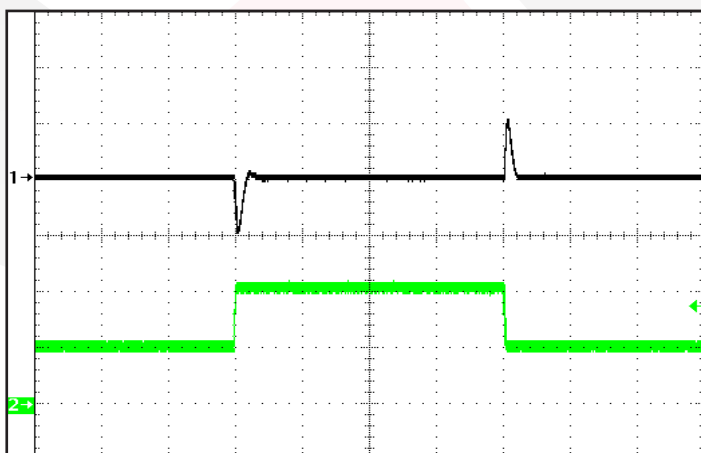
Figure 11: Output voltage response to step-change in load current 50%-100%-50% of I_{out} (max). Load cap: 1 \mu F ceramic cap and 10 \mu F, 100m \Omega ESR tantalum cap. Ch 1: V_{out} (2V/div). Ch 2: I_{out} (2A/div).
