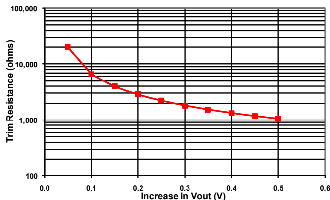
Figure E: Output Voltage Trim Graph
