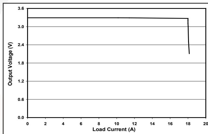
Figure 6: Output voltage vs. load current showing typical current limit curves at V_{in} = 28\text{V} (see Note 4).
