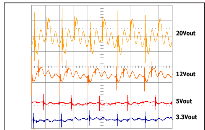
Figure 6: Output Voltage Ripple at 10 V input voltage and rated load current (20mV/div). Zero load capacitance. Bandwidth: 20 MHz (See Figure 4). Timescale: 2 \mu s/div.
