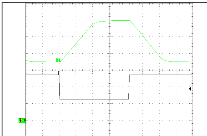
Figure 10: Output Voltage vs. Vset pin voltage dynamics; 28Vin, 2A out (5ms/div). Top trace: Vset pin voltage (500mV/div). Bottom trace: Output Voltage (5V/div).
