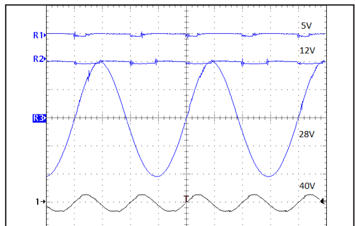
Figure 6: Output Voltage Ripple at 28V input and rated load current (200mV/div). Load capacitance: 100μF electrolytic cap. Bandwidth: 20MHz, (2uS/div). See Figure 4.
