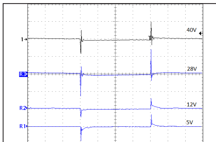
Figure 14: Output voltage response for 28V input; 5V, 12V, 28V, 40V output to step change in load current (50%-75%-50% pf lout max; di/dt=0.1A/uS). Vout (1V/div); (5mS/div)
