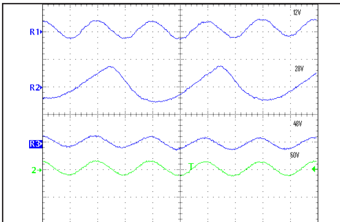
Figure 5: Input Terminal Ripple Current at 28V input and rated load current (500mA/div). Load capacitance: 100 \mu F electrolytic cap. Bandwidth: 20MHz, (2 \mu S/div). See Figure 4
