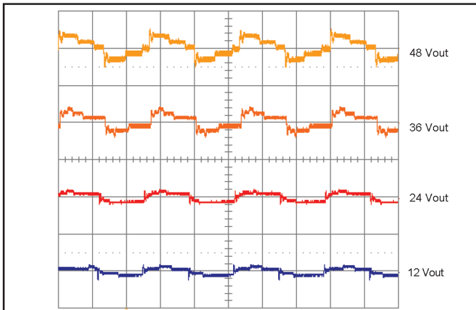
Figure 11: Output voltage response for 12V, 24V, 36V, and 48Vout to step-change in load current (50-75-50% of Iout max; di/dt=0.1A/μs). Load cap: 100μF, 100mΩ ESR tant, Vout (2V/div). Timescale: 5 ms/div.
