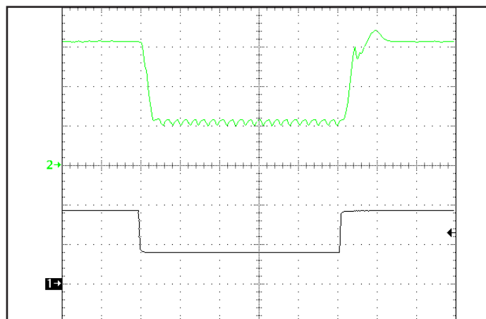
Figure 12: Output Current vs Iset pin voltage dynamics; 28Vin 10Vout (2mS/div). Top Trace: Output Current (5A/div). Bottom Trace: Iset pin voltage (500mV/div).
