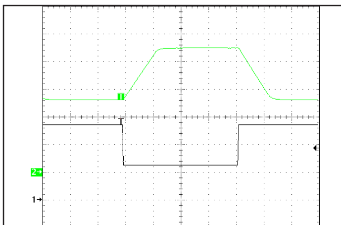
Figure 10: Output Voltage vs. Vset pin voltage dynamics; 28Vin, 5A out (10ms/div). Bottom trace: Vset pin voltage (500mV/div). Top trace: Output Voltage (10V/div).
