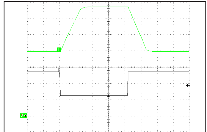
Figure 10: Output Voltage vs. Vset pin voltage dynamics; 48Vin, 2A out (10mS/div). Bottom trace: Vset pin voltage (500mV/div). Top trace: Output Voltage (10V/div).
