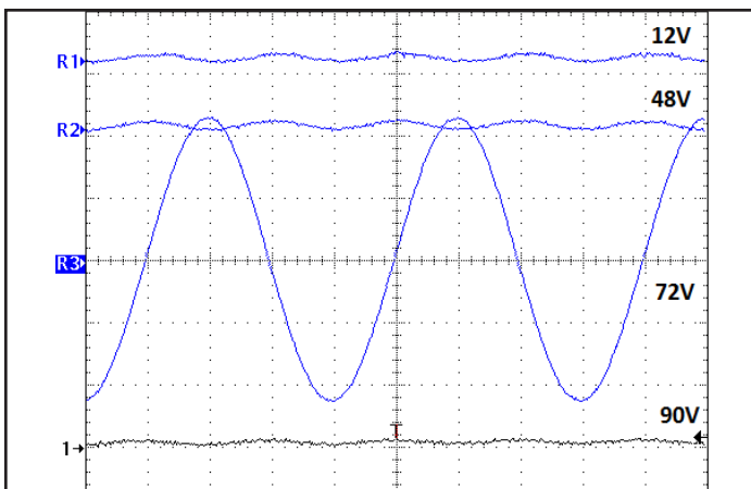
Figure 5: Input Terminal Ripple Current at 48V input and rated load current (50mA/div). Load capacitance: 100μF electrolytic cap. Bandwidth: 20MHz (See Figure 4). Timescale: 2 μs/div.
