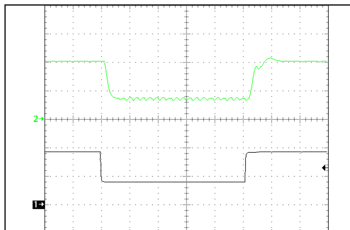
Figure 12: Output Current vs I_{set} pin voltage dynamics at 48V input and 10V output. Ch2: Output Current (5A/div), Ch1: I_{set} pin voltage (500mV/div). Timescale: 2 ms/div.
