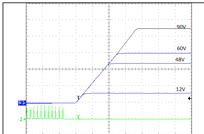
Figure 8: Turn-on transient at 48V input and zero load. Top Traces: V_{out} (20V/div), Ch2: ON/OFF input (5V/div). Timescale: 5 ms/div.
