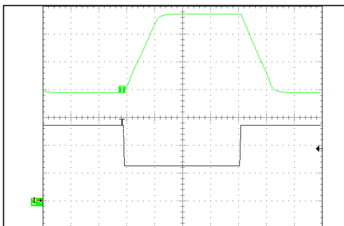
Figure 10: Output Voltage vs. V_{set} pin voltage dynamics at 48V input and 2A output. Ch2: Output Voltage (10V/div), Bottom trace: V_{set} pin voltage (500mV/div). Timescale: 5 ms/div.
