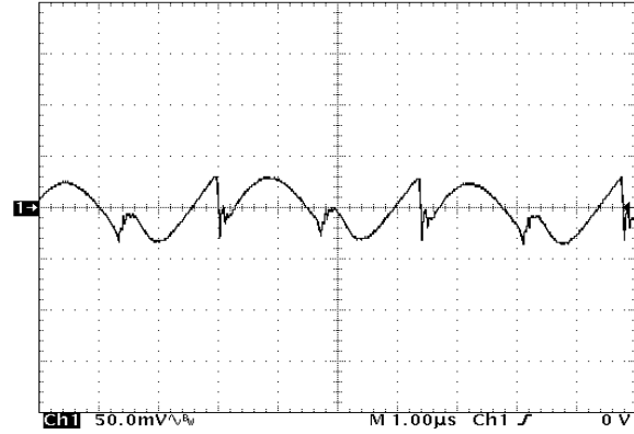
Figure 20: Output voltage ripple at nominal input voltage and rated load current (50 mV/div). Load capacitance: 1 \mu\text{F} ceramic capacitor and 10 \mu\text{F} tantalum capacitor. Bandwidth: 20 MHz. See Figure 17.
