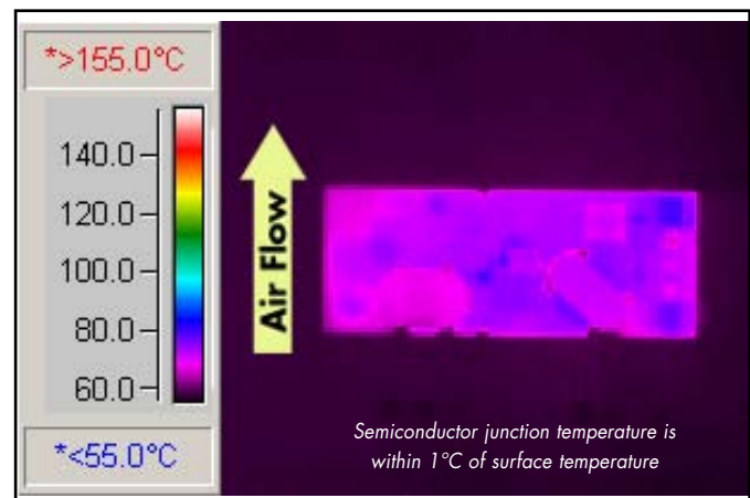
Figure 6: Thermal plot of converter at 15 amp load current with 55°C air flowing at the rate of 200 LFM. Air is flowing across the converter from pin 3 to pin 1 (nominal input voltage).
