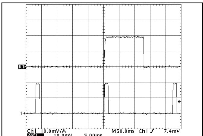
Figure 18: Load current (10A/div) as a function of time when the converter attempts to turn on into a 10\ \text{m}\Omega short circuit. Top trace (5.0ms/div) is an expansion of the on-time portion of the bottom trace.
