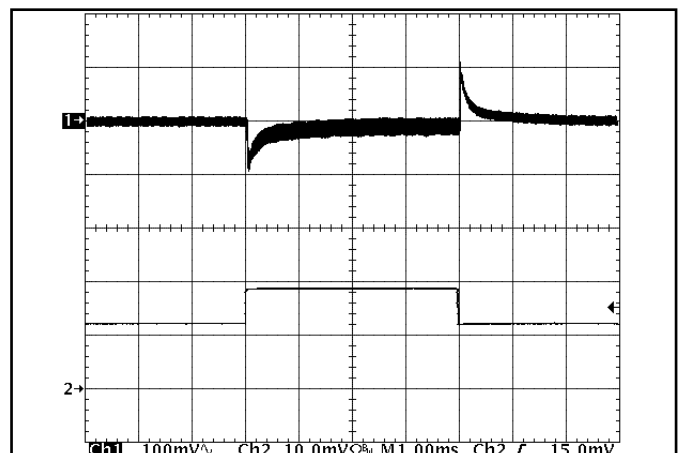
Figure 12: Output voltage response to step-change in load current (50%-75%-50% of I_{out(max)} ; dl/dt = 5A/\mu s ). Load cap: 470 \mu F , 30 m \Omega ESR tantalum cap and 1 \mu F ceramic cap. Ch 1: V_{out} (100mV/div), Ch 2: I_{out} (10A/div).
