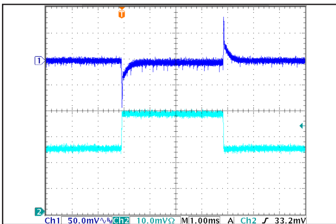
Figure 5: Output voltage response to step-change in load current (50%-75%-50% of Iout(max)); dI/dt = 0.1A/us. Load cap: 15µF tantalum cap and 1µF ceramic cap. Ch 1: Vout(50.0mV/div), Ch 2: Iout(10.0mA/div). Time scale(1.00ms/div).
