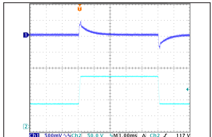
Figure 6: Output voltage response to step-change in input voltage (650V/ms), at Max. load current. Load cap: 15µF tantalum cap and 1µF ceramic cap. Ch 1: Vout(500mV/div), Ch 2: Vin(50.0V/div). Time scale(1.00ms/div).
