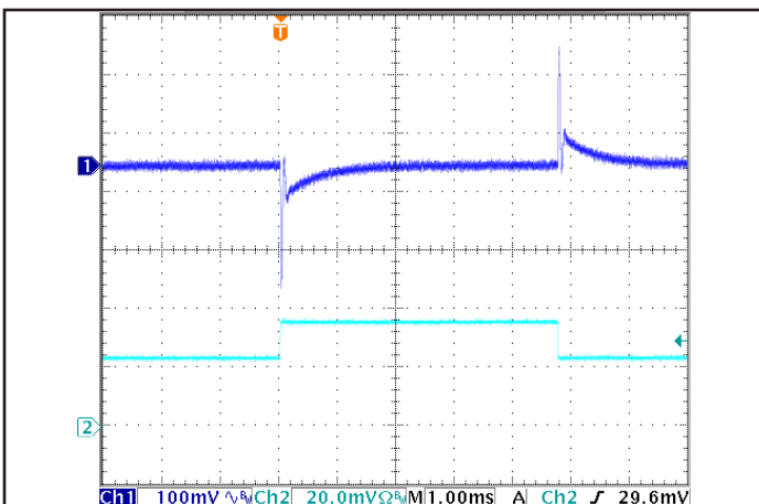
Figure 5: Output voltage response to step-change in load current (50%-75%-50% of Iout(max); di/dt = 0.1A/us. Load cap: 15µF tantalum cap and 1µF ceramic cap. Ch 1: Vout(100mV/div), Ch 2: Iout(20.0mA/div). Time scale(1.00ms/div).
