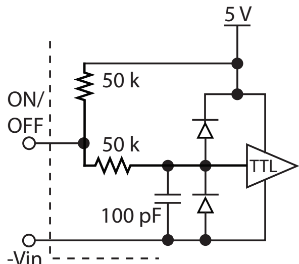
Figure B: Internal ON/OFF pin circuitry
