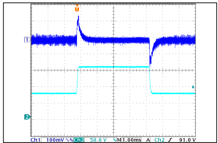
Figure 6: Output voltage response to step-change in input voltage (715V/ms), at Max. load current. Load cap: 15µF tantalum cap and 1µF ceramic cap. Ch 1: Vout(100mV/div), Ch 2: Vin(50.0V/div). Time scale(1.00ms/div).
