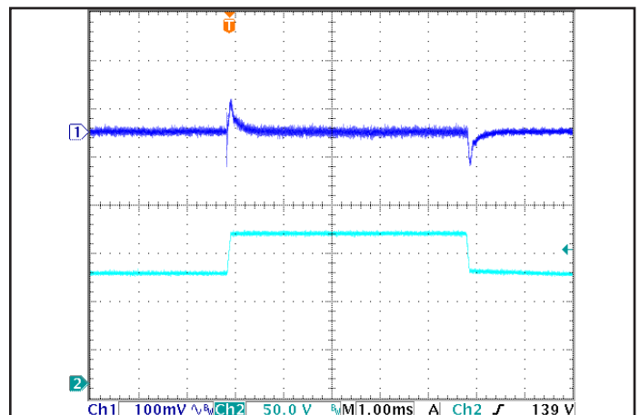
Figure 6: Output voltage response to step-change in input voltage (600 V/ms), at Max. load current. Load cap: 1 μF ceramic cap. Ch 1: Vout(100mV/div), Ch 2: Vin (50.0V/div). Time scale(1.00ms/div).
