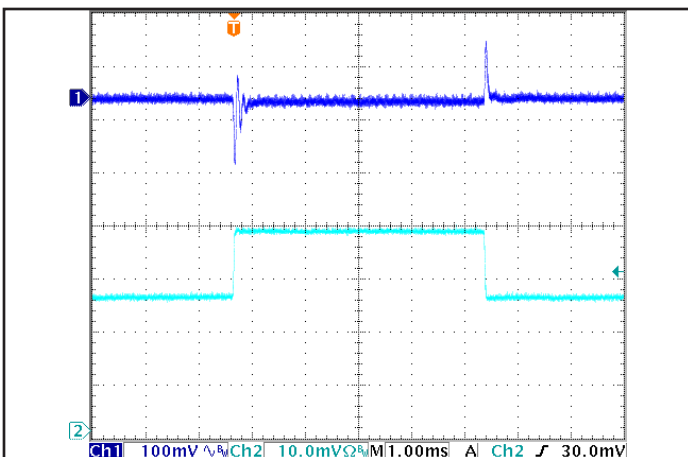
Figure 5: Output voltage response to step-change in load current (50%-75%-50% of Iout(max); dI/dt = 0.1 A/μs). Load cap: 1 μF ceramic and 15 μF tantalum capacitors. Ch 1: Vout(100mV/div), Ch 2: Iout(10.0mA/div). Time scale(1.00ms/div).
