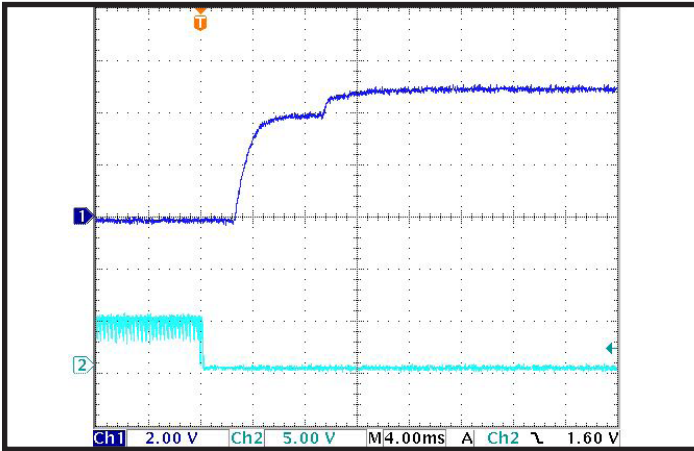
Common Figure 1: Typical startup waveform on Ch 1 (2.00V/div). Input voltage pre-applied, ON/OFF Pin on Ch 2 (5.00V/div). Time scale (4.00ms/div).
