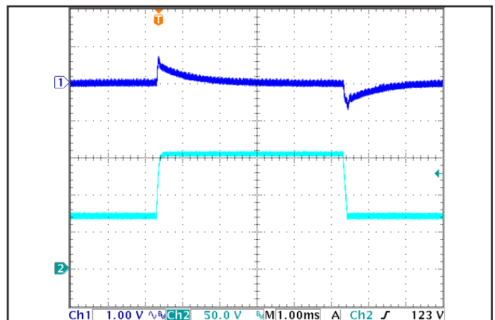
Figure 6: Output voltage response to step-change in input voltage (1000 V/ms). Load cap: 1 μF ceramic and 15 μF tantalum capacitors. Ch 1: Vout(1.00V/div), Ch 2: Vin(50.0V/div). Time scale(1.00ms/div).
