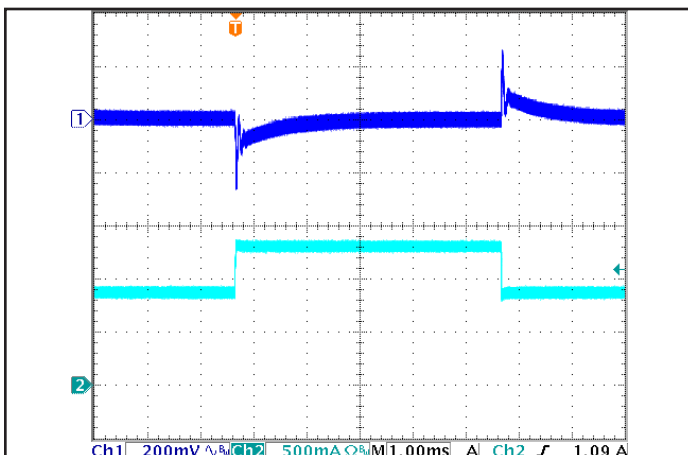
Figure 5: Output voltage response to step-change in load current (50%-75%-50% of Iout(max); dI/dt = 0.1 A/μs). Load cap: 1 μF ceramic and 15 μF tantalum capacitors. Ch 1: Vout(200mV/div), Ch 2: Iout(500mA/div). Time scale(1.00ms/div).
