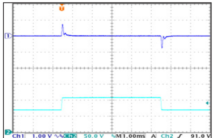
Figure 6: Output voltage response to step-change in input voltage (1V/ms). Load cap: 1 μF ceramic and 15 μF tantalum capacitors. Ch 1: V out , Ch 2: V in .
