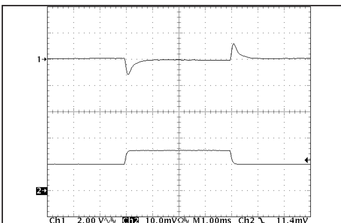
Figure 11: Output voltage response to step-change in load current (50%-75%-50%) of I out (max); dI/dt = 0.1 A/μs. Load cap 100 μF, 100 mΩ ESR tantalum cap. Top trace: Vout (2 V/div), Ch2: Iout (10A/div). Vin = 48 V
