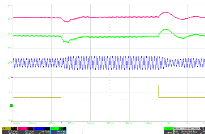
Figure 5: Load transient with 600μF hold-up capacitor (50%-75%-50% of I_{max} , 115Vrms, 60Hz) Ch1: Iout (10A/div), Ch2: Hold-up voltage (100V/div), Ch3: Iin (20A/div), Ch4: Vout (5V/div), Timebase: (200ms/div).
