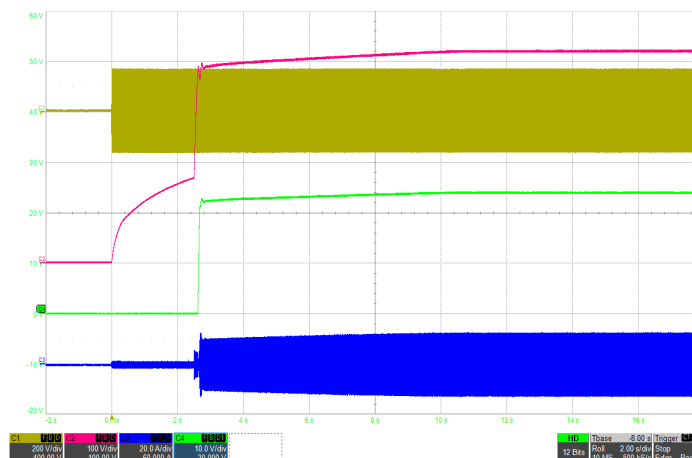
Figure 4: Typical startup waveform with 600μF hold-up capacitor (115Vrms, 400Hz) Ch1: Vin (200V/div), Ch2: Hold-up capacitor voltage (100V/div), Ch3: Iin (20A/div), Ch4: Vout (10V/div), Timebase: (2s/div).
