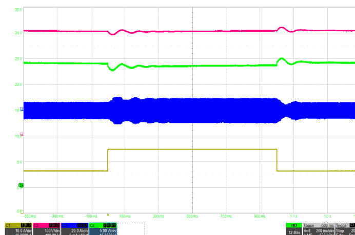
Figure 6: Load transient with 600μF hold-up capacitor (50%-75%-50% of I_{max} , 115Vrms, 400Hz) Ch1: Iout (10A/div), Ch2: Hold-up voltage (100V/div), Ch3: Iin (20A/div), Ch4: Vout (5V/div), Timebase: (200ms/div).
