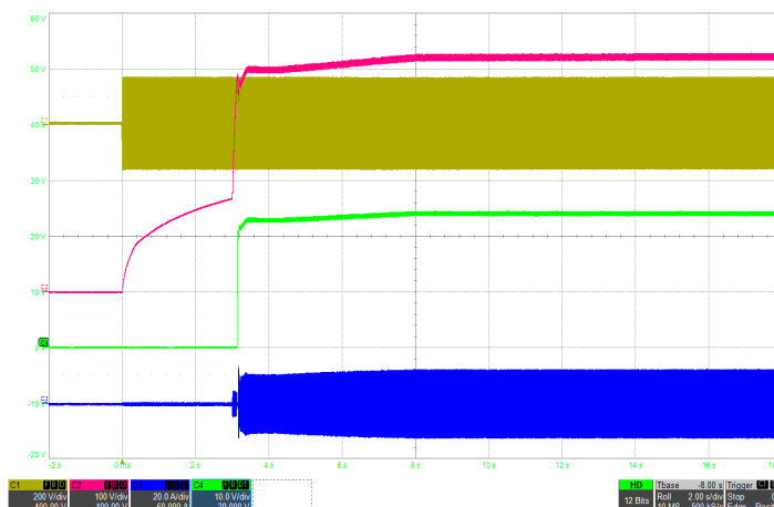
Figure 3: Typical startup waveform with 600μF hold-up capacitor (115Vrms, 60Hz) Ch1: Vin (200V/div), Ch2: Hold-up capacitor voltage (100V/div), Ch3: Iin (20A/div), Ch4: Vout (10V/div), Timebase: (2s/div).
