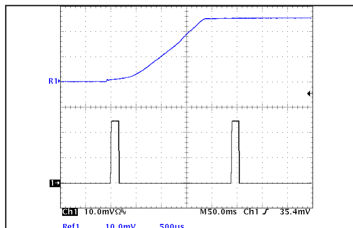
Figure 18: Load current (50A/div) as a function of time when the converter attempts to turn on into a 1mΩ short circuit. Top trace (500□s/div) is an expansion of the on-time portion of the bottom trace.
