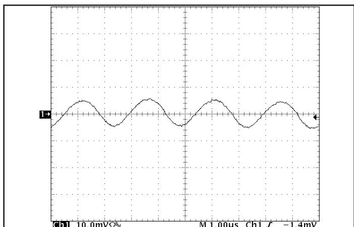
Figure 15: Input reflected ripple current, i_s , at nominal input voltage and rated output current through a 10µH source inductor, using a 47µF electrolytic input capacitor (20mA/div). See Figure 13.
