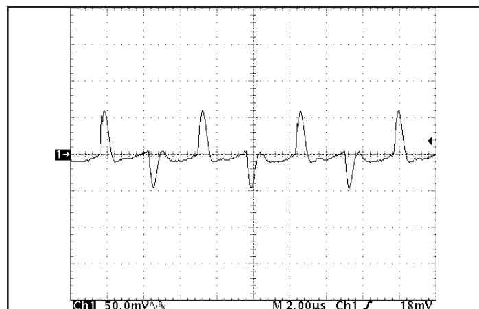
Figure 16: Output voltage ripple at nominal input voltage and rated load current (50mV/div). Load capacitance: 1µF ceramic capacitor and 15µF tantalum capacitor. Bandwidth: 20MHz. See Figure 13.
