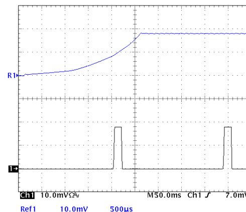
Figure 18: Load current (50 A/div) as a function of time when the converter attempts to turn on into a 1 mΩ short circuit. Top trace (500 µs/div) is an expansion of the on-time portion of the bottom trace.
