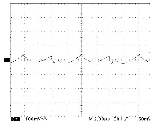
Figure 16: Output voltage ripple at nominal input voltage and rated load current (100 mV/div). Load capacitance: 1 µF ceramic capacitor and 15 µF tantalum capacitor. Bandwidth: 20 MHz. See Figure 13.
