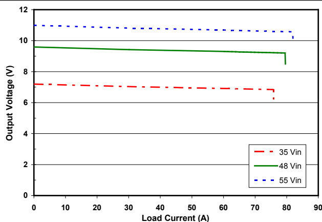
Figure 17: Output voltage vs. load current for different input voltages showing typical current limit curves.
