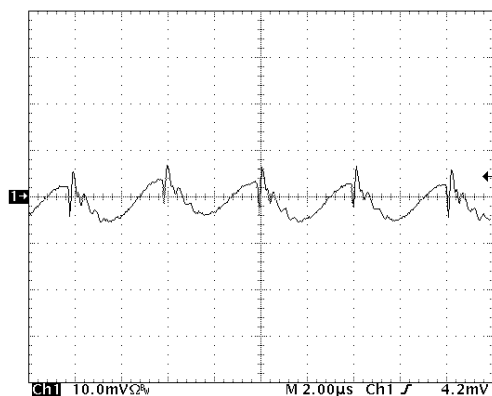
Figure 15: Input reflected ripple current, i_s , through a 10 µH source inductor, using a 47 µF electrolytic input capacitor (50 mA/div). See Figure 13.
