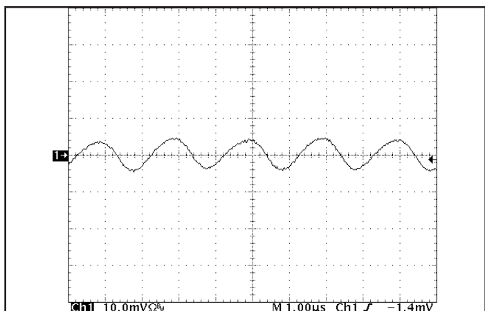
Figure 15: Input reflected ripple current, i_s , at nominal input voltage and full rated output current through a 10µH source inductor, using a 47µF electrolytic input capacitor (20mA/div). See Figure 13.
