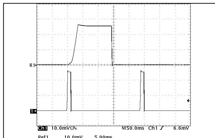
Figure 18: Load current (50A/div) as a function of time when the converter attempts to turn on into a 1mΩ short circuit. Top trace (5ms/div) is an expansion of the on-time portion of the bottom trace.
