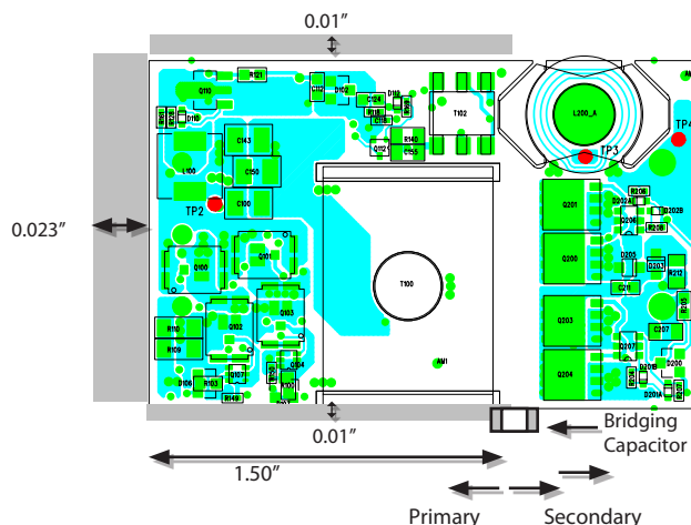
Figure F: Keep Out Areas for BusQor module (open frame)
