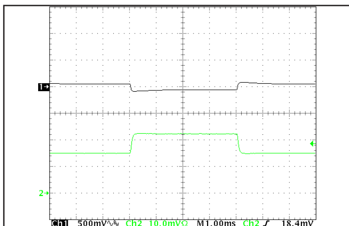
Figure 11: Output voltage response to step-change in load current (50%-75%-50% of I_{out(max)} ; dI/dt = 0.1 A/ \mu s). Load cap: 15 \mu F tantalum cap and 1 \mu F ceramic cap. Ch 1: V_{out} (500 mV/div), Ch 2: I_{out} (20 A/div).
