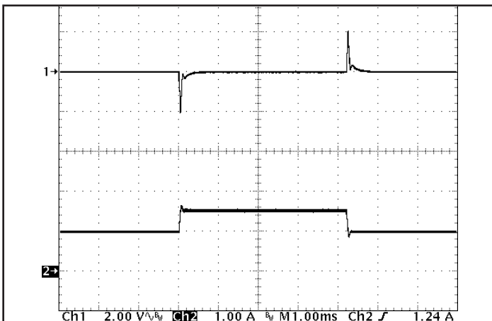
Figure 5: Output voltage response to step-change in load current (50% -75% -50% of I_{out(max)} ; dI/dt = 0.1 A/\mu s ). Load cap: 1 \mu F ceramic capacitor. Ch 1: V_{out} (2 V/div), Ch 2: I_{out} (1 A/div).
