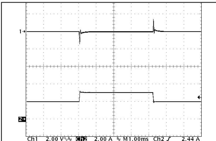
Figure 5: Output voltage response to step-change in load current (50% -75% -50% of I out (max); dI/dt = 0.1 A/μs). Load cap: 1 μF ceramic cap. Ch 1: V out (2 V/div), Ch 2: I out (2 A/div).
