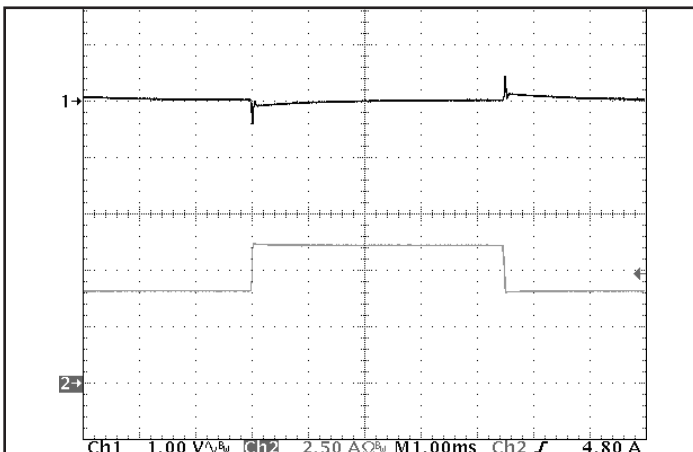
Figure 5: Output voltage response to step-change in load current (50% - 75% - 50% of I out (max); dI/dt = 0.1 A/μs). Load cap: 15 μF tantalum cap and 1 μF ceramic cap. Ch 1: V out (1 V/div), Ch 2: I out (2.5 A/div).
