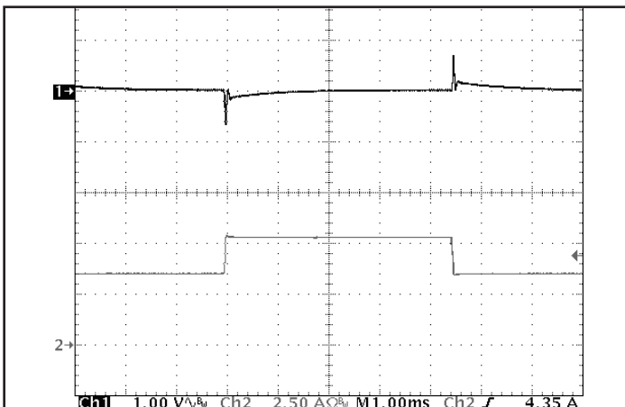
Figure 5: Output voltage response to step-change in load current (50% -75% -50% of Iout(max); dI/dt = 0.1 A/μs). Load cap: 15 μF tantalum cap and 1 μF ceramic cap. Ch 1: Vout (1 V/div), Ch 2: Iout (2.5 A/div).
