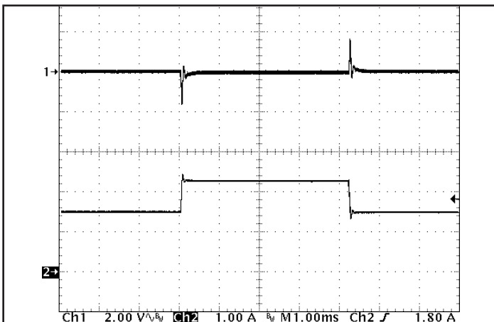
Figure 5: Output voltage response to step-change in load current (50% -75% -50% of Iout(max); dI/dt = 0.1 A/μs). Load cap: 1 μF ceramic cap. Ch 1: Vout (2 V/div), Ch 2: Iout (1 A/div).
