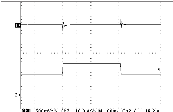
Figure 5: Output voltage response to step-change in load current (50% -75% -50% of I out (max); dI/dt = 0.1 A/μs). Load cap: 15 μF tantalum cap and 1 μF ceramic cap. Ch 1: V out (500 mV/div), Ch 2: I out (10 A/div).
