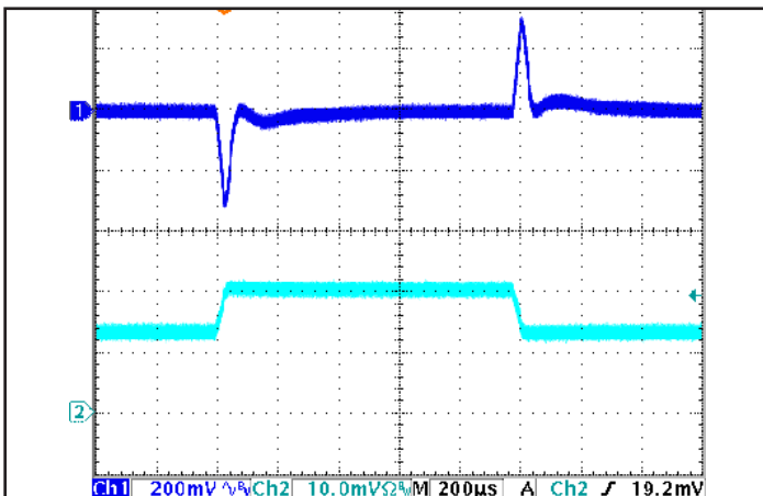
Figure 5: Output voltage response to step-change in load current (50% -75% -50% of I out (max); dI/dt = 0.1 A/μs). Load cap: 15 μF tantalum cap and 1 μF ceramic cap. Ch 1: V out (200 mV/div), Ch 2: I out (5 A/div).
