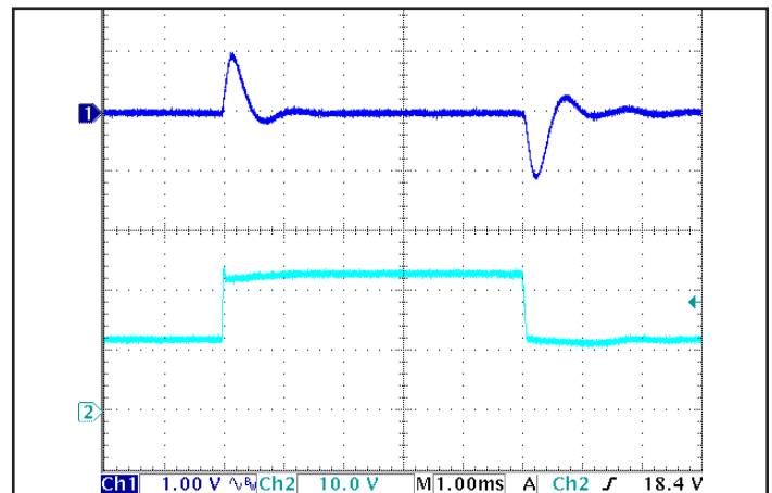
Figure 6: Output voltage response to step-change in input voltage (nominal to maximum, 250 V/ms). Load cap: 1 \mu F ceramic capacitor. Ch 1 V_{out} (1 V/div); , Ch 2: V_{in} (10 V/div).
