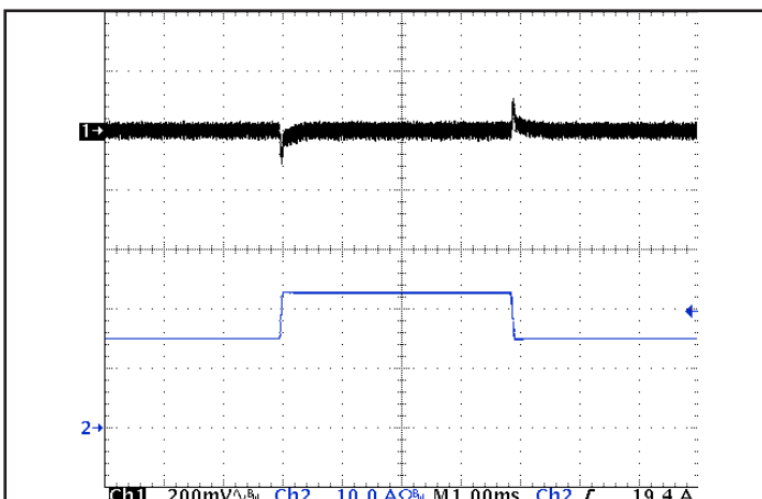
Figure 5: Output voltage response to step-change in load current (66 % -100 % -66 % of I out (max); dI/dt = 0.1 A/μs). Load cap: 15 μF tantalum cap and 1 μF ceramic cap. Ch 1: V out (200 mV/div), Ch 2: I out (10 A/div).
