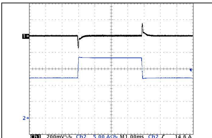
Figure 5: Output voltage response to step-change in load current (66 % -100 % -66 % of I out (max); dI/dt = 0.1 A/μs). Load cap: 15 μF tantalum cap and 1 μF ceramic cap. Ch 1: V out (200 mV/div), Ch 2: I out (5 A/div).
