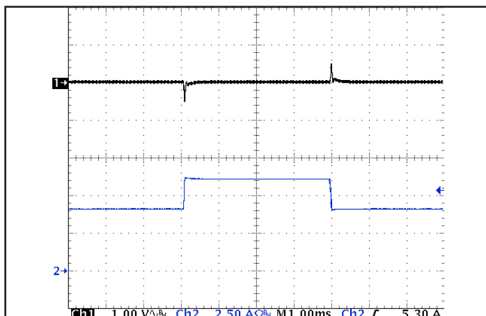
Figure 5: Output voltage response to step-change in load current (66 % -100 % -66 % of Iout(max); dI/dt = 0.1 A/μs). Load cap: 15 μF tantalum cap and 1 μF ceramic cap. Ch 1: Vout (1 V/div), Ch 2: Iout (2.5 A/div).
