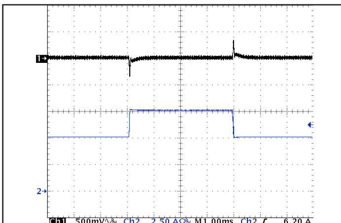
Figure 5: Output voltage response to step-change in load current (66 % -100 % -66 % of I out (max); dI/dt = 0.1 A/μs). Load cap: 15 μF tantalum cap and 1 μF ceramic cap. Ch 1: V out (500 mV/div), Ch 2: I out (2.5 A/div).
