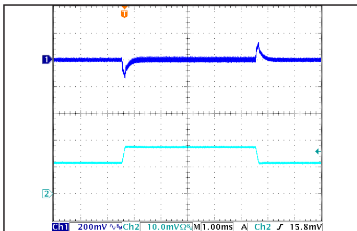
Figure 5: Output voltage response to step-change in load current (50 % -75 % -50 % of I out (max); dI/dt = 0.1 A/μs). Load cap: 15 μF Tantalum + 1 μF Ceramic capacitor. Ch 1: V out , Ch 2: I out (20 A/div).
