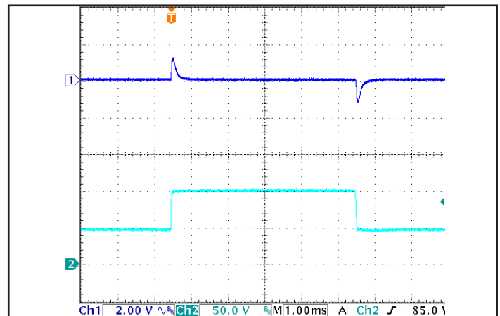
Figure 6: Output voltage response to step-change in input voltage (nominal to maximum, 250 V/ms). Load cap: 1 uF ceramic capacitor. Ch 1: V out , Ch 2: V in .
