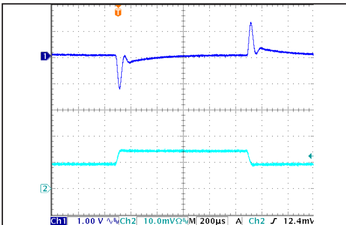
Figure 5: Output voltage response to step-change in load current (66% -100% -66% of I out (max); dI/dt = 0.2 A/μs). Load cap: 1 uF ceramic capacitor. Ch 1: V out (1 V/div), Ch 2: I out (5 A/div).
