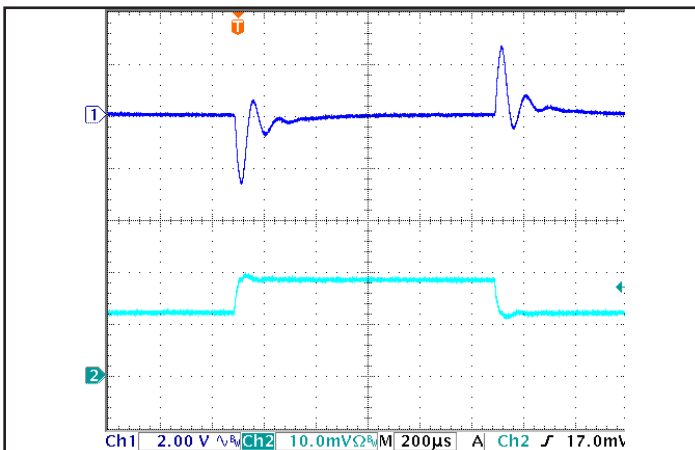
Figure 5: Output voltage response to step-change in load current (66% -100% -66% of I out (max); dI/dt = 0.2 A/μs). Load cap: 1 uF ceramic capacitor. Ch 1: V out (2 V/div), Ch 2: I out (2 A/div).
