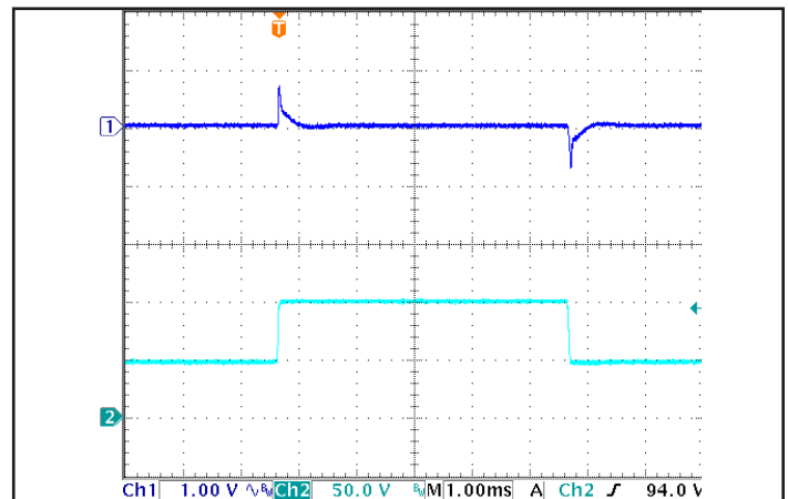
Figure 6: Output voltage response to step-change in input voltage (nominal to maximum, 250 V/ms). Load cap: 15 µF tantalum and 1 µF ceramic capacitors. Ch 1: V out , Ch 2: V in .
