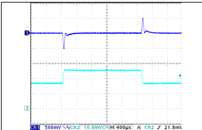
Figure 5: Output voltage response to step-change in load current (66% -100% -66% of I out (max); dI/dt = 0.2 A/μs). Load cap: 15 μF tantalum and 1 μF ceramic capacitors. Ch 1: V out (500 mV/div), Ch 2: I out (5 A/div).
