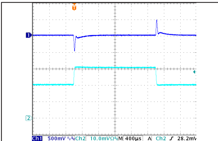
Figure 5: Output voltage response to step-change in load current (66% -100% -66% of I out(max) ; dI/dt = 0.2 A/us). Load cap: 15 µF tantalum and 1 µF ceramic capacitors. Ch 1: V out (500 mV/div), Ch 2: I out (5 A/div).
