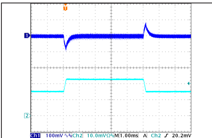
Figure 5: Output voltage response to step-change in load current (66% -100% -66% of Iout(max); dI/dt = 0.2 A/μs). Load cap: 15 μF tantalum and 1 μF ceramic capacitors. Ch 1: Vout (100 mV/div), Ch 2: Iout (20 A/div).
