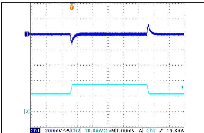
Figure 5: Output voltage response to step-change in load current (66% -100% -66% of I out (max); dI/dt = 0.2 A/μs). Load cap: 15 μF tantalum and 1 μF ceramic capacitors. Ch 1: V out (200 mV/div), Ch 2: I out (20 A/div).
