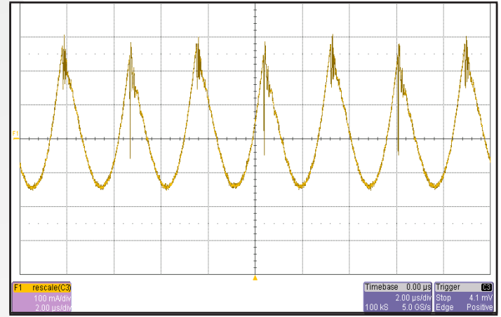
Figure 16: Input terminal ripple, i_c , at full load and nominal input voltage with 10 \mu H source impedance and 100 \mu F electrolytic capacitor (100 mA/div). Bandwidth: 20 MHz. See Figure 12. Timebase: 2.00 \mu s /div.
