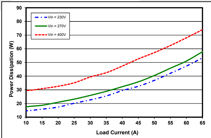
Figure 3: Power dissipation vs. load current for minimum, nominal, and maximum input voltage at T_{CASE}=25^{\circ}\text{C} .
