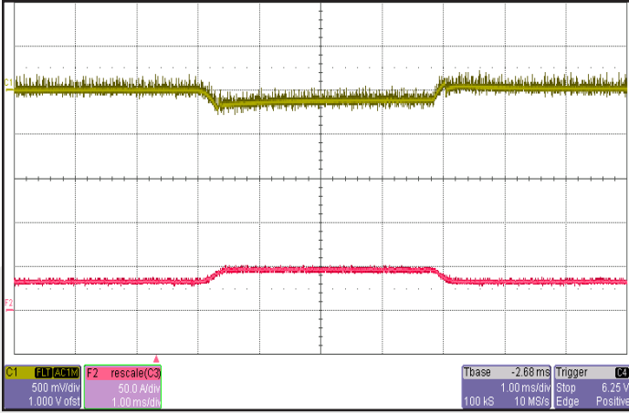
Figure 13: Output voltage response to step-change in load current 50%-75%-50% of I_{out(max)} ; dI/dt = 0.1 A/\mu s . Load capacitance: 1 \mu F ceramic and 15 \mu F 100 m \Omega ESR tantalum. Ch1: V_{out} (500 mV/div). Ch 2: I_{out} (50 A/div). Timebase: 1.00 msec/div.
