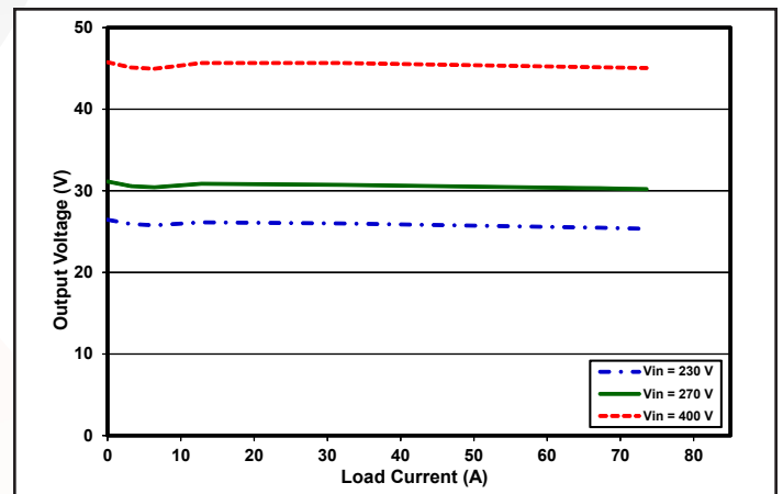
Figure 6: Output voltage vs. load current, current limit curves for minimum, nominal, and maximum input voltage at T_{CASE}=25^{\circ}\text{C} .
