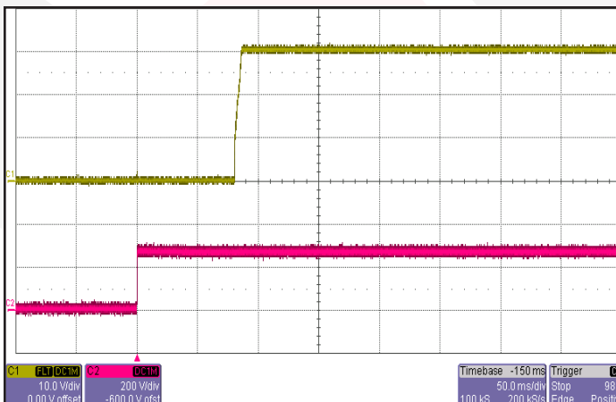
Figure 11: Turn-on transient at half resistive load and 100 \mu\text{F} output capacitance initiated by V_{in} . ENA previously enabled. Ch 1: V_{out} (10 V/div). Ch 2: V_{in} (200 V/div). Timebase: 50.0 msec/div.
