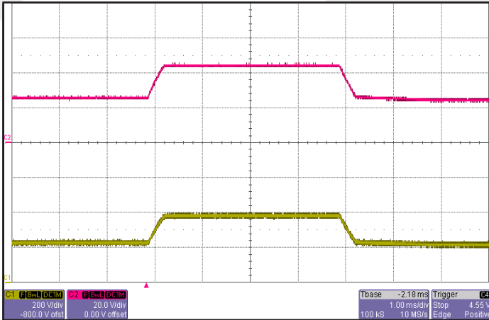
Figure 15: Output voltage response to step-change in input voltage 230V-400V-230V in 250us. Load capacitance: 10 \mu F , 100 m \Omega ESR tantalum cap and 1 \mu F ceramic cap. Ch1: V_{in} (200 V/div), Ch2: V_{out} (20 V/div). Timebase: 1.00 msec/div.
