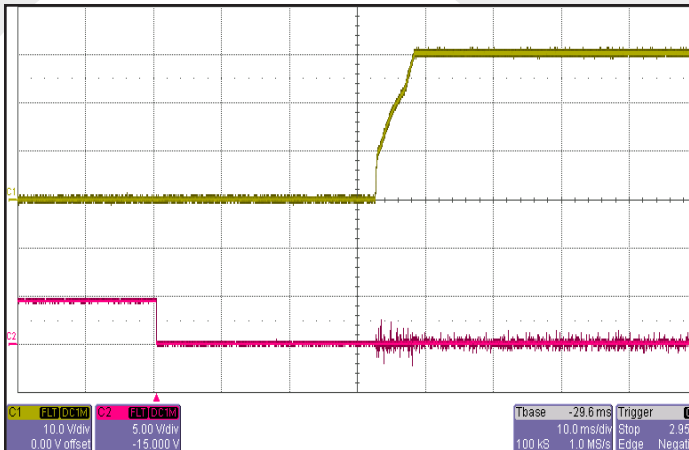
Figure 9: Turn-on transient at half resistive load and 100 \mu\text{F} output capacitance initiated by ENA. Input voltage pre-applied. Ch 1: V_{out} (10 V/div). Ch 2: ENA (5 V/div). Timebase: 10.0 msec/div.
