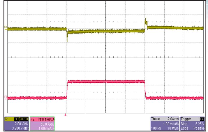
Figure 14: Output voltage response to step-change in load current 10%-100%-10% of I_{out(max)} . Load capacitance: 1 \mu F ceramic and 15 \mu F 100 m \Omega ESR tantalum. Ch1: V_{out} (2 V/div). Ch 2: I_{out} (50 A/div). Timebase: 1.00 msec/div.
