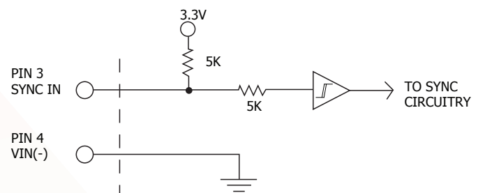
Figure C: Equivalent circuit looking into the SYNC IN pin with respect to the IN RTN (input return) pin.
